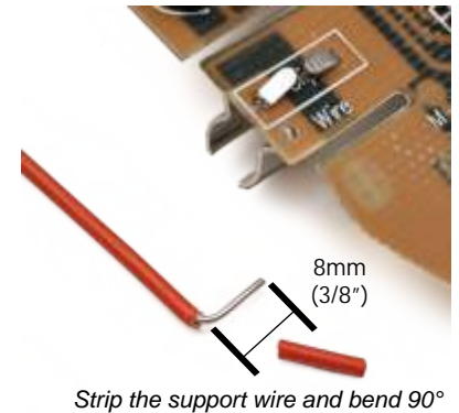
Strip the support wire and bend 90°
