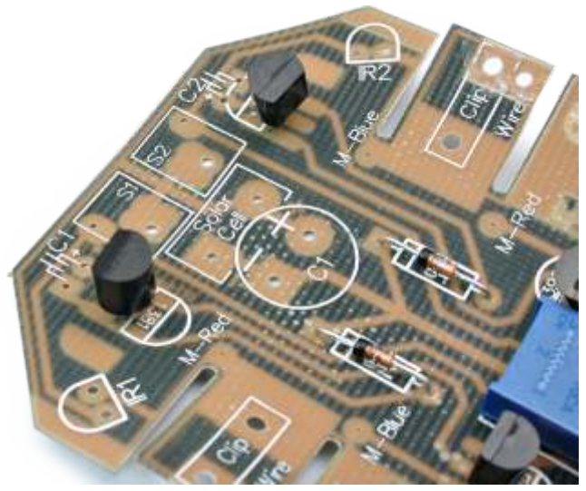
Close-up of the 1381 and diodes installed on the PCB. Note the directions that these parts are facing - they don't work when installed backwards!
