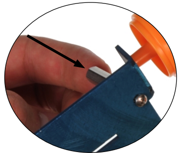
Hex stand-offs are mounted with #4-40 x 3/8" bolts
