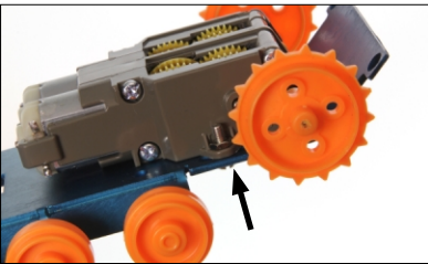
Pocket nut in mounting tab, bolt from underneath
