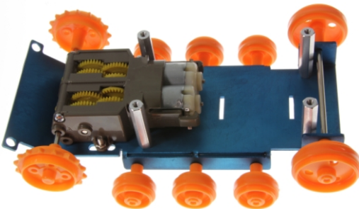
Complete pre-tread Assembly
